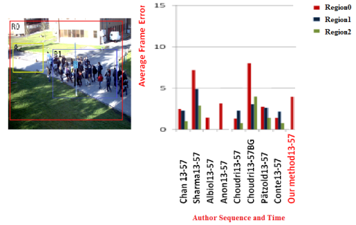
Figure 5: Counting People Evaluation
