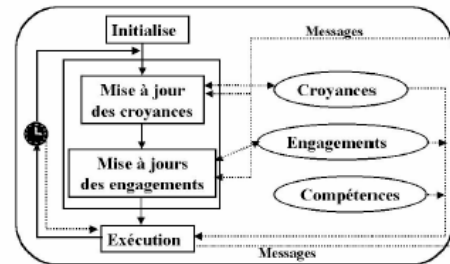
AOP (Agent Oriented Programming) [Shoham 93]
