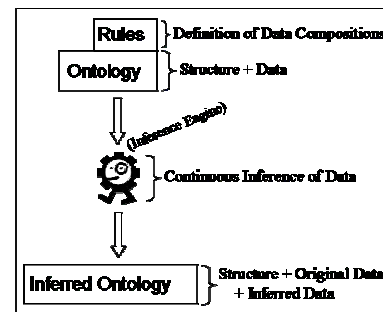
Fig. 1. The DynaCROM composition process
