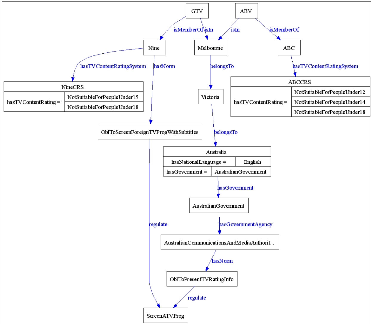
Fig. 3. An instance part of the conceptual model for norm appliance and management in our television NMA
